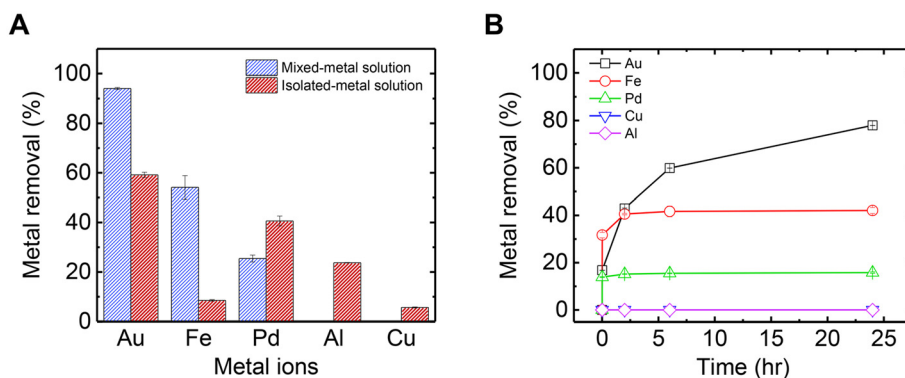
Fig. 1 (A) Metal removal by mucin from mixed-metal and isolated-metal aqueous solutions (initial concentration of each metal: 0.05 mM in steady state). (B) Removal of all metals by mucin as a function of time from an aqueous mixed-metal solution containing 0.05 mM of each metal. All experiments were conducted in 0.1 \text{g L}^{-1} dissolved mucin and solution pH of 4. Error bars represent one standard deviation from an average of two measurements.
