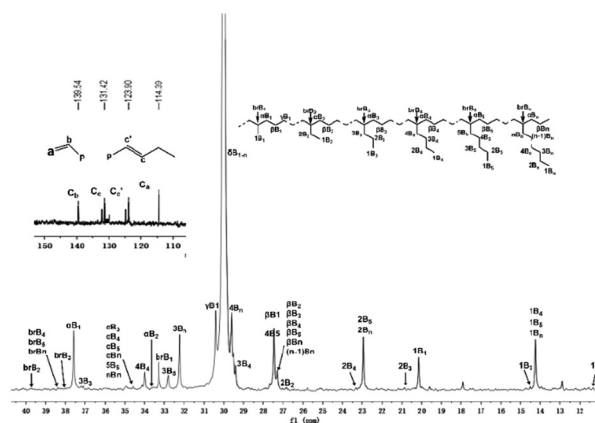
Fig. 10 ^{13}\text{C} NMR spectrum of the polyethylene sample produced using Ni5 /EASC at 20 °C (entry 5, Table 4) together with an inset showing the \delta 114–140 region and a segment of the assigned polymer backbone recorded at 110 °C in 1,1,2,2-tetrachloroethane- d_2 .
