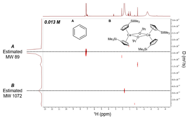
Fig. 4 2D ^1\text{H} DOSY NMR spectra of 0.013 M 2-Ce/ i Pr in \text{C}_6\text{D}_6 demonstrating preservation of dimer in solution.
