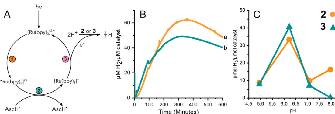
Fig. 3 (A) Reaction scheme for photoactivated HER. (B) \text{H}_2 produced by 2 (a, orange) and 3 (b, teal) at pH 6.2 under photocatalytic conditions. Detection by \text{H}_2 sensing electrode. (C) \text{H}_2 detected in headspace at reaction completion under a range of pH conditions.
