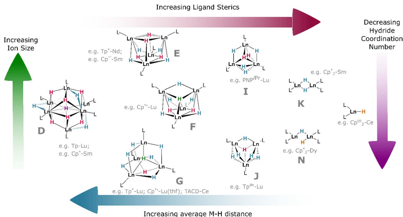
Fig. 9 Trends in structures of Ln hydride clusters with examples of L and Ln for each set. Ligand abbreviations: \text{Cp}^{\bullet} = \text{C}_5(\text{CH}_3)_5 ; \text{Cp}^{\bullet\bullet} = \text{C}_5(\text{CH}_3)_4(\text{SiMe}_3) ; \text{Cp}^{\text{ttt}} = \text{C}_5\text{H}_2(\text{tBu})_3 ; \text{Tp}^{\bullet} = \text{tris}(3,5\text{-dimethylpyrazolyl})\text{borane} ; \text{Tp}^{\text{IPr}} = \text{tris}(3\text{-isopropyl-5-methylpyrazolyl})\text{borane} ; \text{PNP}^{\text{IPr}} = \text{N}(\text{o-C}_6\text{H}_4\text{P}^{\text{IPr}})_2 ; TACD = \kappa^4\text{-N,N,N,N-Me}_4\text{-1,4,7,10-tetraazadodecane} .
