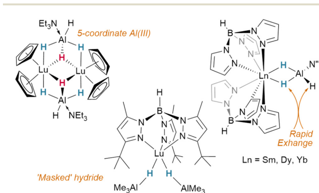
Fig. 16 Examples of aluminohydride complexes of lanthanides.
