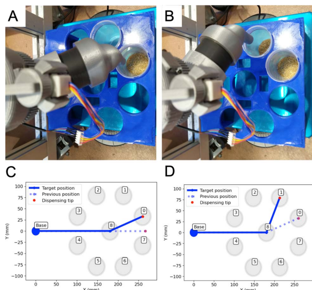
Fig. 10 Demonstration of the working principle of the pellet distributor. (A) The distributor tip is over a cup number 0. (B) When the required amount of material is detected by the balance, the tip moves to cup 1. (C and D) Represents the Inverse Kinematics calculation of the movement between starting position and cup 0 (C) and between cup 0 and 1 (D). The program calculates the rotation of the joints needed to reach the desired positions.
