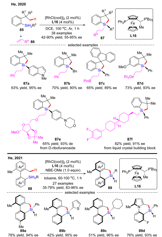
Scheme 26 Rh(I)-Catalyzed asymmetric silylation of unactivated C(sp^3)-H bonds.
