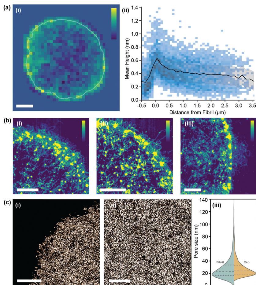
Fig. 2 Network-wide structural characteristics of kDNA molecules. (a) (i). Mean image height of single molecule with 300 nm sample resolution sample. Scale bar: 2 \mu m, Height scale: 2 nm. (ii). Mean image height against distance from fibril for 15 molecules. (b) High contrast height images of close-ups of the outer fibril. Scale bar: 200 nm. Height scale: 1–4 nm. (c) (i) and (ii). Binary images highlighting pores in the network. Scale bar: 500 nm. (iii). Pore size distribution for near-fibril and interior cap.
