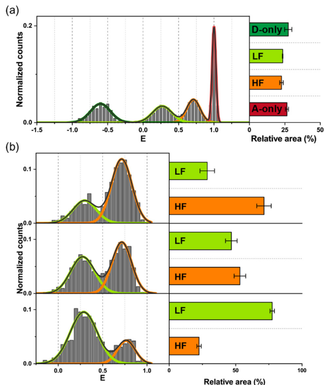
Fig. 6 (a) The E histogram for a mixture of D-only, A-only, HF, and LF samples of 10 pM each, constructed with \gamma = 1.84 using four Gaussian fits for the D-only (green), A-only (red), LF (yellow green) and HF (orange) samples. (b) E histograms of 1 : 3 (10 pM LF, 30 pM HF), 2 : 2 (20 pM LF, 20 pM HF) and 3 : 1 (30 pM LF, 10 pM HF) mixture samples constructed with \gamma = 1.84 using two Gaussian fits for the LF (yellow green) and HF (orange) samples. Black lines are the sum of Gaussian fits. The relative area under each Gaussian function is shown on the right side of the E histogram. The error bars of the relative areas were calculated using the standard deviations of the three experiments.
