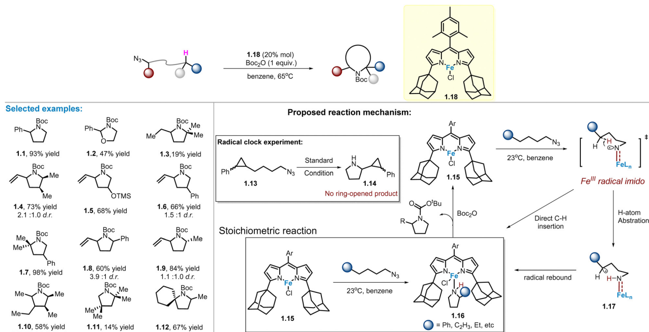
Scheme 1 \text{Fe}(\text{III}) -dipyrrinato-catalysed intramolecular \text{C}(\text{sp}^3)\text{-H} amination of alkyl azides.
