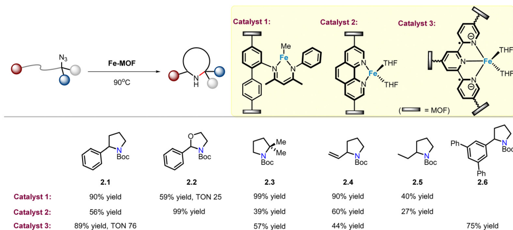
Scheme 2 MOF supported iron catalysts for intramolecular \text{C}(\text{sp}^3)\text{-H} amination of alkyl azides.
