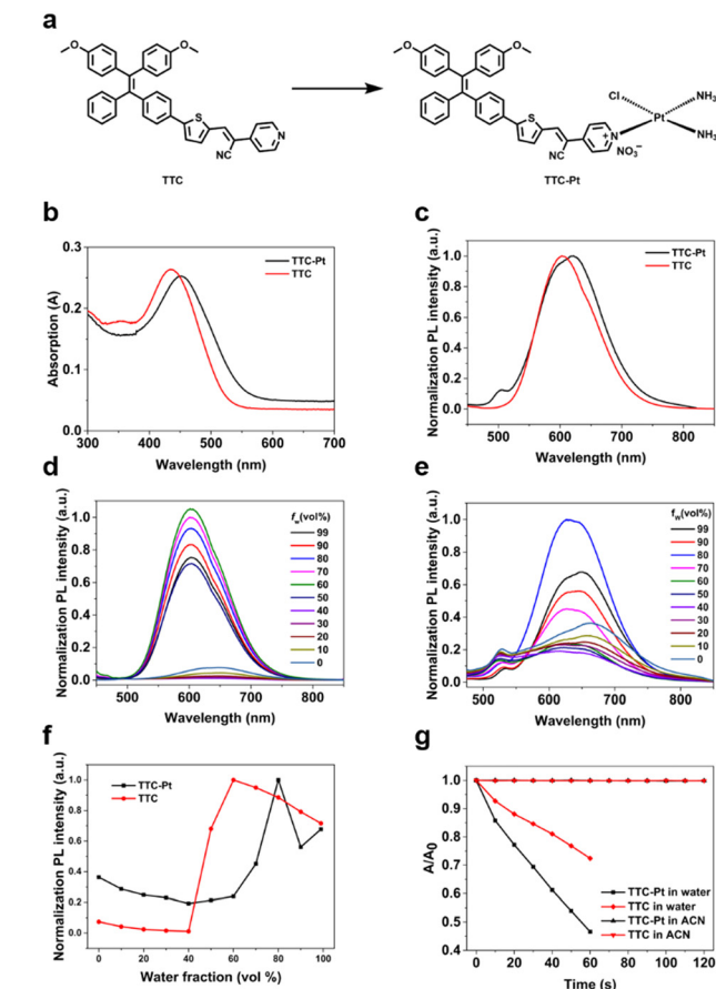
Fig. 1 (a) Chemical structures of TTC and TTC-Pt. (b) Absorption and (c) emission spectra of TTC and TTC-Pt (10 \mu\text{M} ) were measured in water (containing 1% DMSO, v/v). Emission spectra of the AIEgens (10 \mu\text{M} ) including (d) TTC and (e) TTC-Pt in the mixed solvents of DMSO and water with different water fractions ( f_w ). (f) Emission intensity plot of TTC-Pt and TTC in different f_w of the solvent mixture. (g) The decomposition rates of ABDA in the presence of TTC-Pt under illumination in different solvents ( A_0 and A represent the absorption of ABDA before and after irradiation, respectively).
