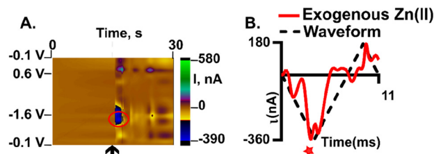
Fig. 7 Exogenous detection of 200 \mu\text{M} Zn(II). (A) False color plot showing injection of Zn(II) and duration of event. (B) “Open” CV of associated false color plot showing reduction of Zn(II) denoted by a red star. n = 3 .
