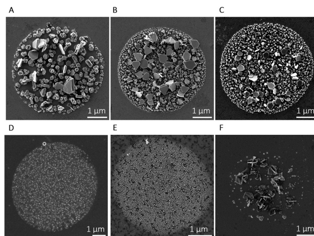
Fig. 2 Representative SEM images of AgNP spots obtained via SECCM using pipettes with a diameter of \sim 5 \mu\text{m} , on a 25-cycle PDA film. The applied potentials were kept constant ( E_1 = -0.4 V and E_2 = -0.2 V vs. Ag/AgCl). (A) [\text{AgNO}_3] = 5.0 \text{ mmol L}^{-1} , t_1 = 0 s, t_2 = 4.0 s; (B) [\text{AgNO}_3] = 5.0 \text{ mmol L}^{-1} , t_1 = 0.5 s, t_2 = 3.5 s; (C) [\text{AgNO}_3] = 5.0 \text{ mmol L}^{-1} , t_1 = 0.5 s, t_2 = 2.5 s; (D) [\text{AgNO}_3] = 0.5 \text{ mmol L}^{-1} , t_1 = 0.5 s, t_2 = 2.5 s; (E) [\text{AgNO}_3] = 0.05 \text{ mmol L}^{-1} , t_1 = 0.5 s, t_2 = 2.5 s; (F) [\text{AgNO}_3] = 5.0 \text{ mmol L}^{-1} , t_1 = 0.5 s, t_2 = 2.5 s, and 50-cycle PDA film.
