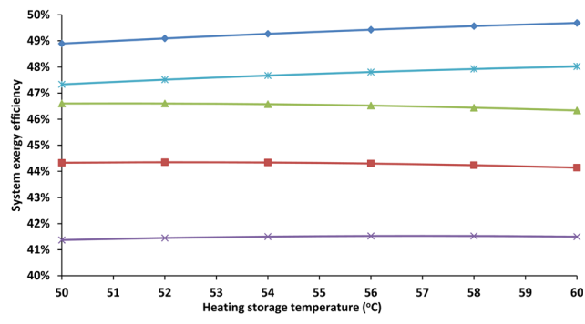
Fig. 7 Overall exergy efficiency depending on the heating storage temperature.
