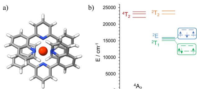
Fig. 4 (a) DFT optimized geometry of the quartet ground state of [Cr(dqp)_2]^{3+} . Spin density at the Cr center: 3.151647. (b) Schematic representation of the energy levels for the calculated (CASSCF(7,12)-FIC-NEVPT2) excited states of [Cr(dqp)_2]^{3+} .
