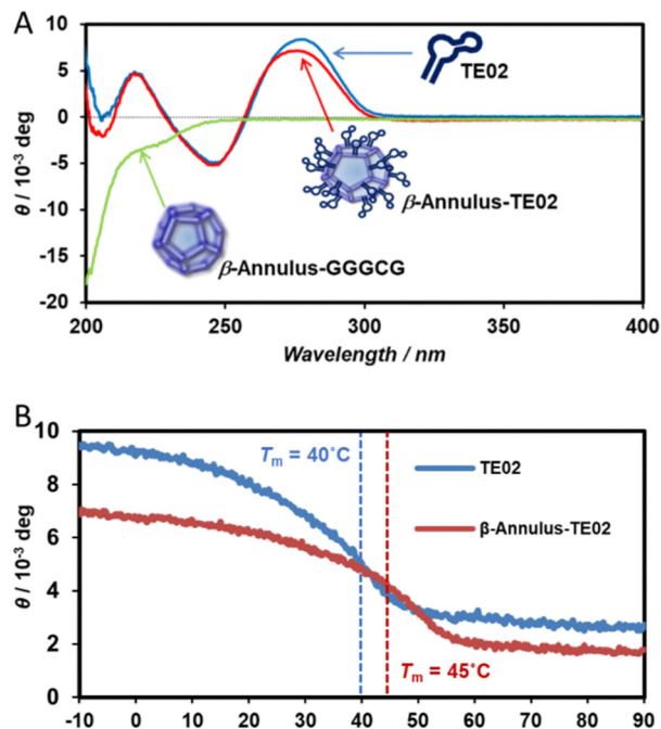
Fig. 3 (A) CD spectra of 20 \mu\text{M} \beta -Annulus-TE02 (red), \beta -Annulus-GGGCG (green), and TE02 (blue) in 10 mM phosphate buffer at 25 ^\circ\text{C} . (B) Temperature-dependence in ellipticity at 270 nm of TE02 (blue) and \beta -Annulus-TE02 (red).
