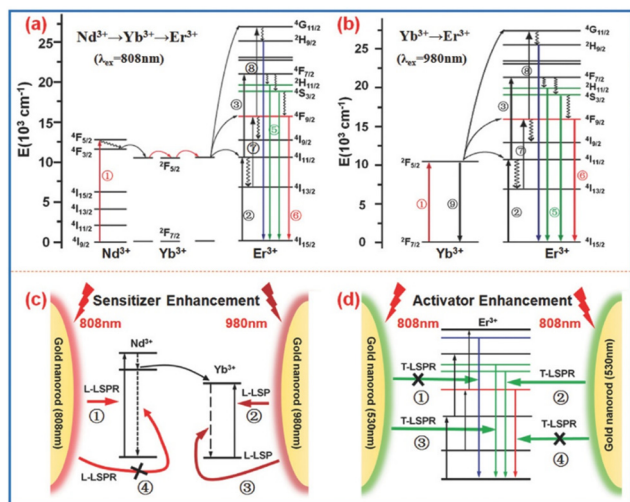
Fig. 3 (a and b) The energy diagrams of Nd 3+ , Yb 3+ , and Er 3+ ions undergoing ETU upon excitation at 808 and 980 nm, respectively. (c) The GNR Longitudinal-LSPR-induced absorption enhancement for an Nd 3+ ion upon excitation at 808 nm and for a Yb 3+ ion upon excitation at 980 nm. The radiative decay rate of the Yb 3+ ion is also accelerated by the GNR Longitudinal-LSPR (due to energy matching) while that of the Nd 3+ ion is not (denoted by “x”) because of the fast phonon-mediated relaxation and energy migration to the Yb 3+ ion. (d) The GNR Transverse-LSPR-induced green-emission enhancement for both ions upon excitation at 808 nm. The blue and red emissions are not affected by the GNR Transverse-LSPR due to energy mismatch (denoted by “x”). 75
