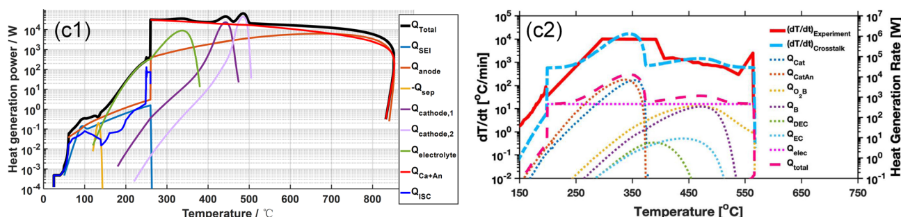
Fig. 4 Thermal runaway modelling of lithium-ion batteries. (a) Fundamental theory for battery TR modelling. (b) Parameterization of the exothermic reactions based on the (b1) ARC and (b2) DSC test data. Reproduced with permission from ref. 39 and 40. Copyright 1999, IOP Publishing, and Copyright 2018, Elsevier. (c) Model-based analysis of the battery TR mechanism. Modified with permission from ref. 41 (c1) and 42 (c2). Copyright 2018, IOP Publishing, and Copyright 2022, Elsevier.
