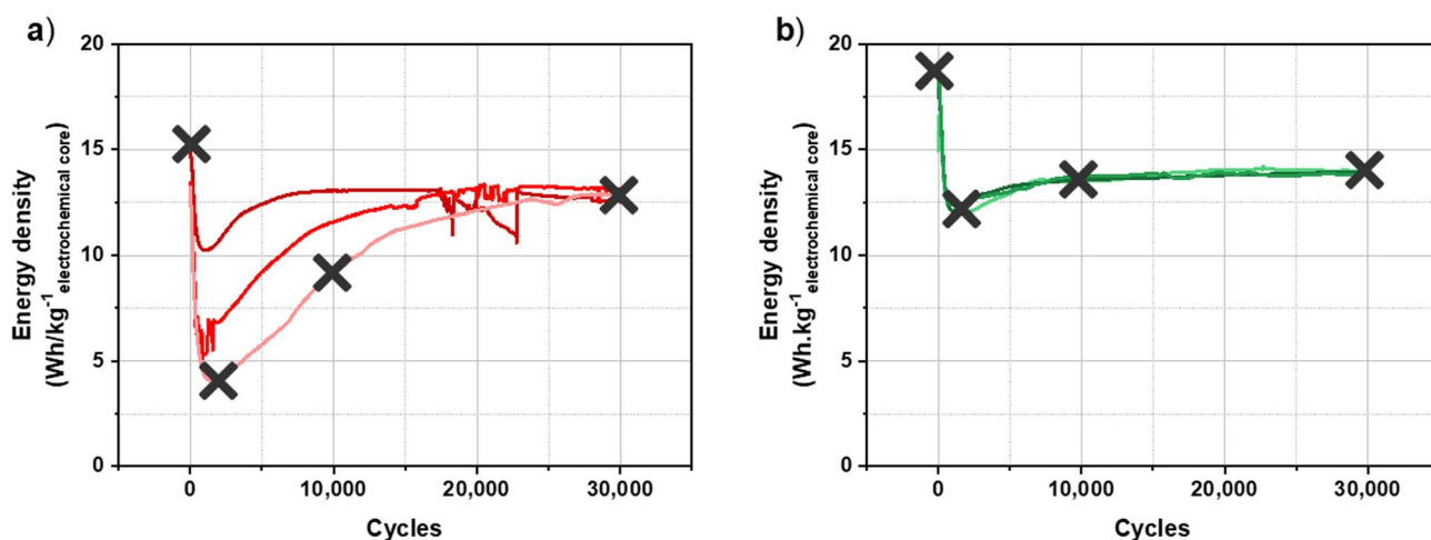
Fig. 5 Long-term cycling of a hybrid KIC in 0.8 \text{ mol L}^{-1} \text{ KPF}_6 AN at 16 \text{ mA cm}^{-2} between 0.5 and 3.5 V at room temperature in the pouch cell configuration after CC formation (a) and after CV formation (b). 8
