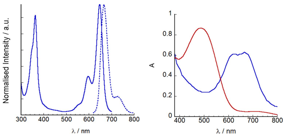
Fig. 5 Left: UV-visible absorption (line) and emission spectra ( \lambda_{ex} = 620 nm, dashed line) of SF5-3 in THF. Right: UV-visible absorption spectra of P1|NiO (red) and SF5-3 |NiO (blue).
