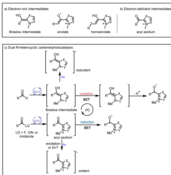
Scheme 1 (a) Typical electron-rich NHC-bound intermediates. (b) Typical electron-deficient NHC-bound intermediates. (c) Main modes of NHC/photoredox dual catalysis.
