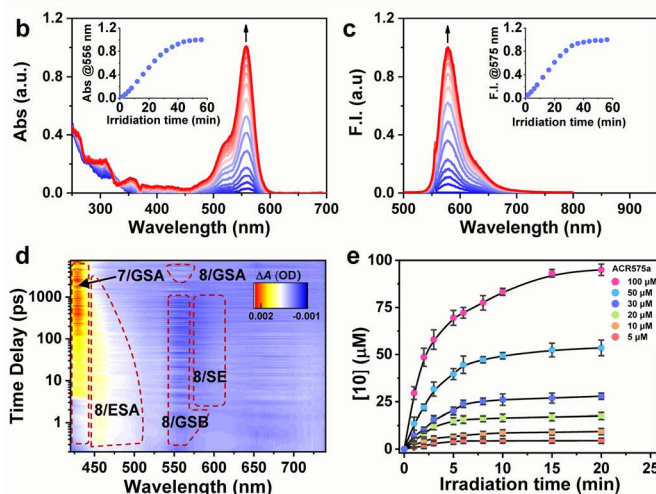
Fig. 3 The molecular design of a photo-triggered acetyl radical donor (ACR575a). (a) The proposed photolysis mechanism of ACR575a. (b) The changes of the UV-vis absorption and (c) fluorescence emission spectra of the ACR575a solution (2 \mu\text{M} ) in phosphate buffer (50 mM, pH = 7.4, with 10% MeCN) upon irradiation by a 375 nm UV light. Inset: absorbance @ 556 nm or fluorescence intensity @ 575 nm along with the irradiation time (min). (d) The femtosecond transient absorption spectra of ACR575a (0–7.48 ns) following a 330 nm laser pump pulse in \text{CH}_3\text{CN} . (e) Fluorescence-based detection of peroxyl radicals generated upon photolysis of ACR575a with a ratiometric probe (light source: a 405 nm laser). (f) The radical trapping chemistry by DMPO upon photolysis of ACR575a. The EPR spectra of ACR575a (1 mM) in \text{CH}_3\text{CN} with DMPO (10 mM) recorded after irradiation with a UV LED light for 8 s or 16 s. (g) The EPR spectrum to confirm the generation of a tertiary benzylic radical (7) without the use of DMPO.
