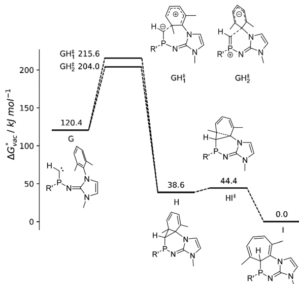
Fig. 5 Free energy profile of the reaction path G \rightarrow I including the identified transition states GH_1^\ddagger and GH_2^\ddagger obtained at B3LYP-GD3BJ/def2-TZVP level of theory in the gas phase. R' = 1,3 -dimethylimidazolin-2-ylidenamino.
