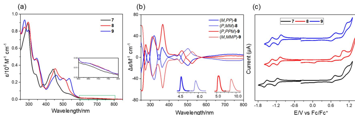
Fig. 5 (a) UV-vis absorption of 7–9 in chloroform ( \sim 10^{-5} \text{ M} ); (b) CD spectra of the enantiomers of 8 and 9 in chloroform. (inset: resolution of the enantiomers of 8 and 9 by chiral analytical HPLC.); (c) cyclic voltammograms of 7–9 in nitrogen-purged dichloromethane with tetrabutylammonium hexafluorophosphate (TBAPF 6 , 0.1 M) as the supporting electrolyte and a scan rate of 100 \text{ mV s}^{-1} .
