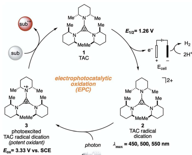
Scheme 10 Electrochemical generation of TAC ^{2+} and photoinduced electron transfer oxidation of substrate by TAC ^{2+*} . Reprinted from ref. 49 with permission from the American Association for the Advancement of Science (Copyright 2021).
