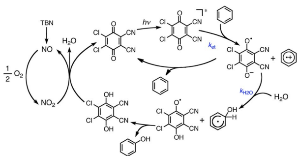
Scheme 7 A mechanism for photohydroxylation of benzene by dioxygen with \text{DDQ} used as a photoredox catalyst in the presence of TBN and \text{H}_2\text{O} in \text{MeCN} under photoirradiation. Reprinted from ref. 44 with permission from American Chemical Society (Copyright 2013).
