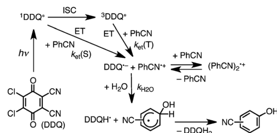
Scheme 8 Proposed mechanism for photohydroxylation of benzonitrile with \text{DDQ} and \text{H}_2\text{O} in \text{MeCN} via ^1\text{DDQ}^* . Reprinted from ref. 47 with permission from John Wiley and Sons (Copyright 2015).
