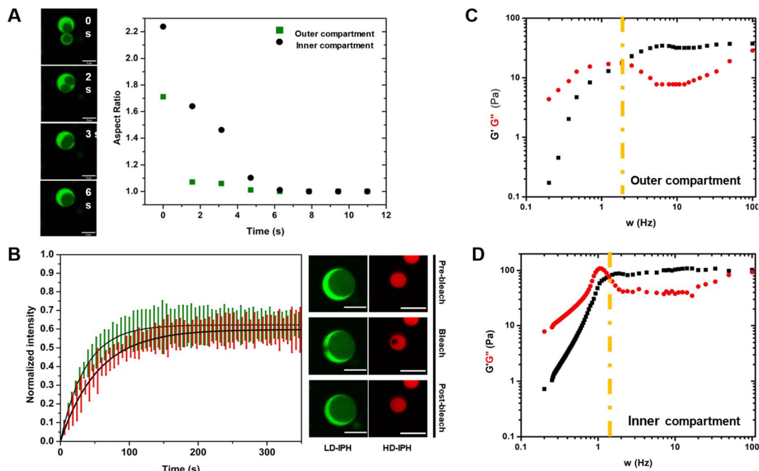
Fig. 3 Biophysical characteristics of multiphase droplets. (A) Images of droplets coalescence and corresponding aspect ratio estimations from fusion events. Aspect ratio for a perfectly spherical shape is equal to 1. Scale bar = 5 \mu\text{m} . (B) FRAP plots (green plot – outer compartment; red – inner compartment) and images showing the fluorescence recovery of multiphase IPH's inner and outer compartments. Scale bar = 10 \mu\text{m} . Plots shown are mean for n = 3 individual droplet measurements per compartment, and their corresponding S.D. (shaded region). (C and D) Linear viscoelastic behaviour of the inner and outer compartments of LD-IPH/HD-IPH/polyU droplets as determined by passive microrheology.
