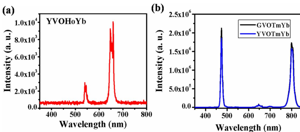
Fig. 4 (a) UC emission spectrum of \text{YVO}_4:\text{Ho}^{3+},\text{Yb}^{3+} phosphor in the range 350–800 nm. (b) UC emission spectra of \text{Tm}^{3+}/\text{Yb}^{3+} co-doped \text{GdVO}_4 and \text{YVO}_4 phosphors in the range from 350–850 nm. ((b) is reproduced with permission from ref. 32 with copyright 2020, Elsevier).
