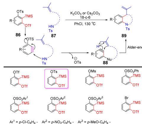
Scheme 15 Domino aryne annulation via a nucleophilic–ene.
