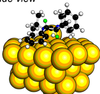
Fig. 4 Binding energies (BE) of NHCs in their energetically favored flat-lying geometry on gold clusters calculated with DFT. (A) represents top view of the NHCs (B) represents the side-view. Black, blue, white, and gold, spheres represent C, N, H, and Au atoms, respectively. The green spheres represent hydrogens bounds to chiral carbons.
