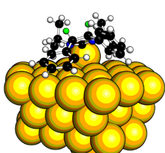
Fig. 4 Binding energies (BE) of NHCs in their energetically favored flat-lying geometry on gold clusters calculated with DFT. (A) represents top view of the NHCs (B) represents the side-view. Black, blue, white, and gold, spheres represent C, N, H, and Au atoms, respectively. The green spheres represent hydrogens bounds to chiral carbons.
