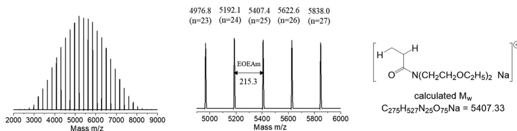
Fig. 2 Matrix assisted laser desorption/ionization-time of flight mass spectrometry (MALDI-TOF MS) spectra of representative PEOEAm with an M_{n,\text{MALS}} of 5.4 \text{ kg mol}^{-1} and an M_w/M_n of 1.20 (Table 1, run 1).
