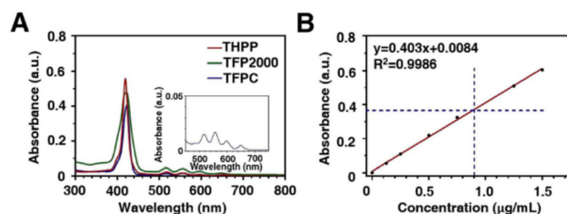
Fig. 1 (A) UV-vis spectra of free THPP ( 1.0\text{ }\mu\text{g mL}^{-1} ), TFP2000 ( 200.0\text{ }\mu\text{g mL}^{-1} ), and TFPC ( 50.0\text{ }\mu\text{g mL}^{-1} ) in ethanol solution. (B) Normalized absorbance of THPP ethanol solution at varying concentrations (detected at 419 nm). The dashed lines mean the THPP porphyrin portion concentrations calculated from the standard curve with the detected UV absorption values of TFPC ethanol solution.
