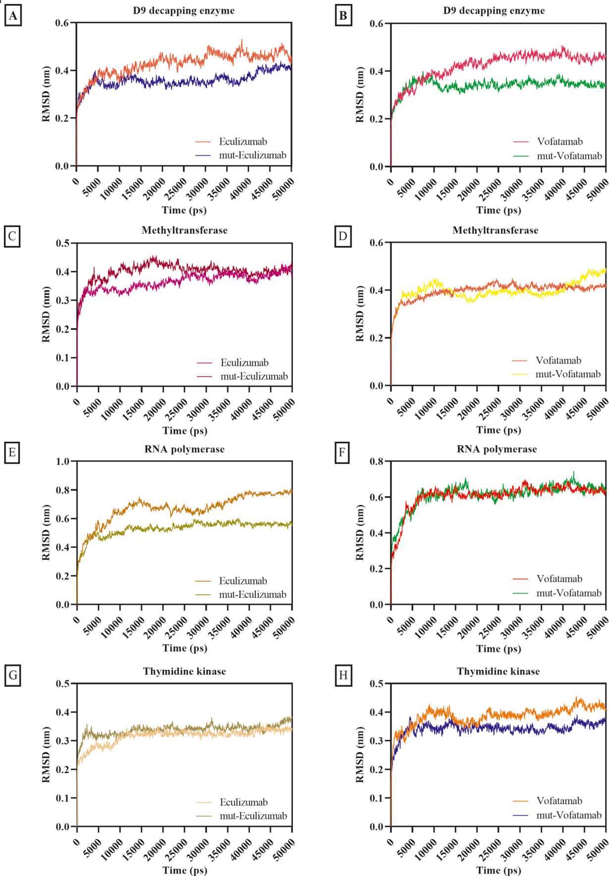
Fig. 3 RMSD plots of D9 decapping enzyme with (A) ecilizumab and ecilizumab mutant (L: L92F), (B) vofatamab mutant (L: H94T, L: Q96V); methyltransferase with (C) ecilizumab and ecilizumab mutant (L: L92F), (D) vofatamab mutant (L: H94T, L: Q96V); RNA polymerase with (E) ecilizumab and ecilizumab mutant (L: L92F), (F) vofatamab mutant (L: H94T, L: Q96V), and thymidine kinase with (G) ecilizumab and ecilizumab mutant (L: L92F), (H) vofatamab mutant (L: H94T, L: Q96V).
