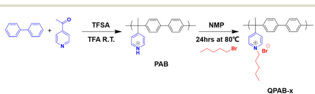
Scheme 1 Synthesis route of poly(alkyl-biphenyl pyridinium) and quaternized poly(alkyl-biphenyl pyridinium).
