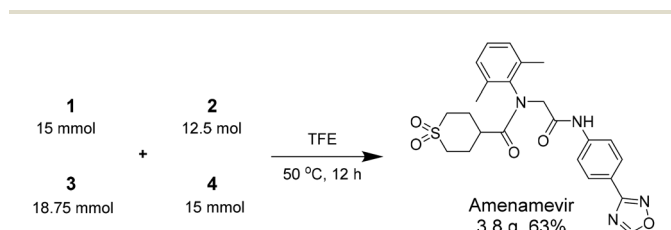
Scheme 1 Gram-scale synthesis.
