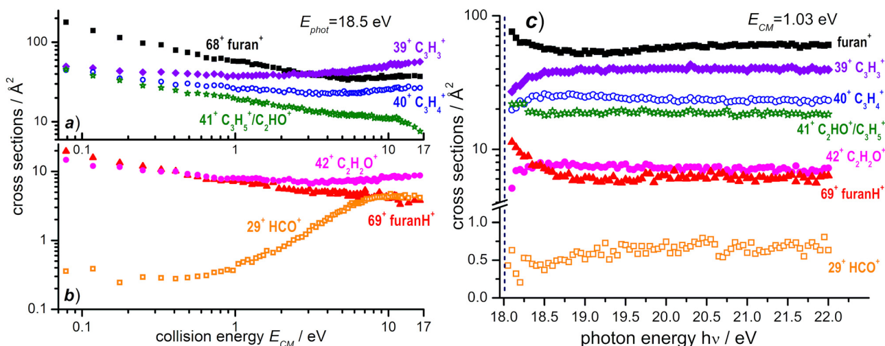
Fig. 8 (a) Absolute reactive cross sections (in log scale) for products 68^+ , 39^+ , 40^+ and 41^+ and (b) for products 69^+ , 29^+ , and 42^+ measured as a function of the collision energy ( E_{\text{CM}} ) from the reaction of \text{OH}^+ with furan, when the former is produced from dissociative photoionization of \text{H}_2\text{O} at a photon energy of 18.50 eV. (c) Absolute reactive cross sections for the same products as in panel (a) and (b) measured at a fixed collision energy E_{\text{CM}} = 1.03 eV as a function of the photon energy. The vertical dashed line (navy color) indicates the AE for the generation of \text{OH}^+ from dissociative photoionization of \text{H}_2\text{O} . Estimated uncertainties on the absolute values of the CSs are about 20%. The error bars are not shown for the sake of clarity.
