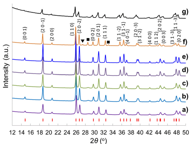
Fig. 1 XRD patterns of (\text{CeTi}_{2.05})_2\text{O}_6 -complex powders calcined for 6 h at (a) 600 °C, (b) 700 °C, (c) 800 °C, (d) 900 °C, (e) 1050 °C, (f) 1150 °C, (g) 1250 °C. The red vertical markers beneath the brannerite patterns show the peak positions expected in the crystal structure. (▼) rutile-type \text{TiO}_2 , (■) \text{CeO}_2 .
