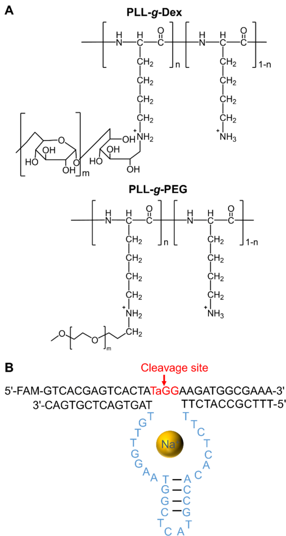
Fig. 1 (A) Chemical structures of cationic copolymers, PLL-g-Dex and poly(L-lysine)-graft-poly(ethylene glycol) (PLL-g-PEG). (B) Secondary structure of EtNa DNase.
