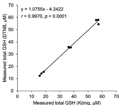
Fig. 5 Correlation between the present method and the DTNB method. Total GSH concentration in the same sample was quantified by the present method (x-axis) and the DTNB method (y-axis). Pearson's correlation analysis was performed.
