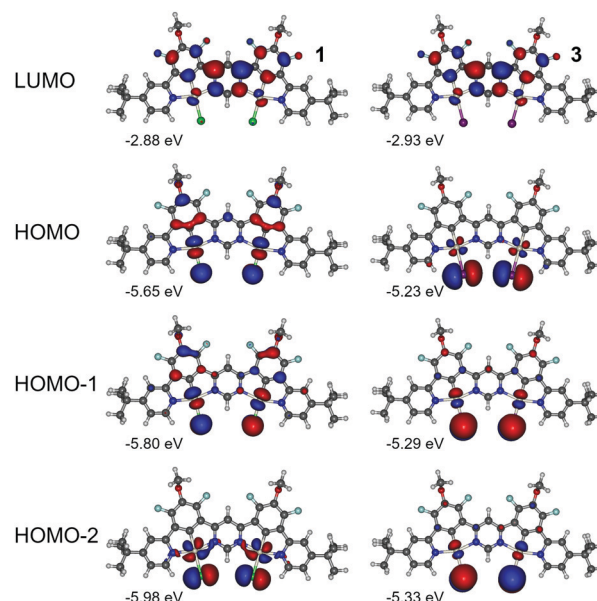
Fig. 8 Molecular orbital contour plots at the B3LYP/dev2-TZVP/ZORA level for diplutonium(II) complexes 1 and 3 .
