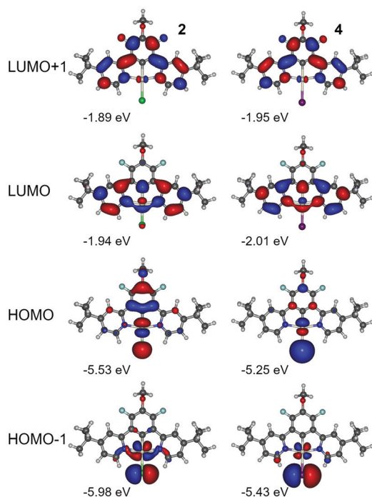
Fig. 7 Molecular orbital contour plots at the B3LYP/dev2-TZVP/ZORA level for monoplutonium(II) complexes 2 and 4 .
