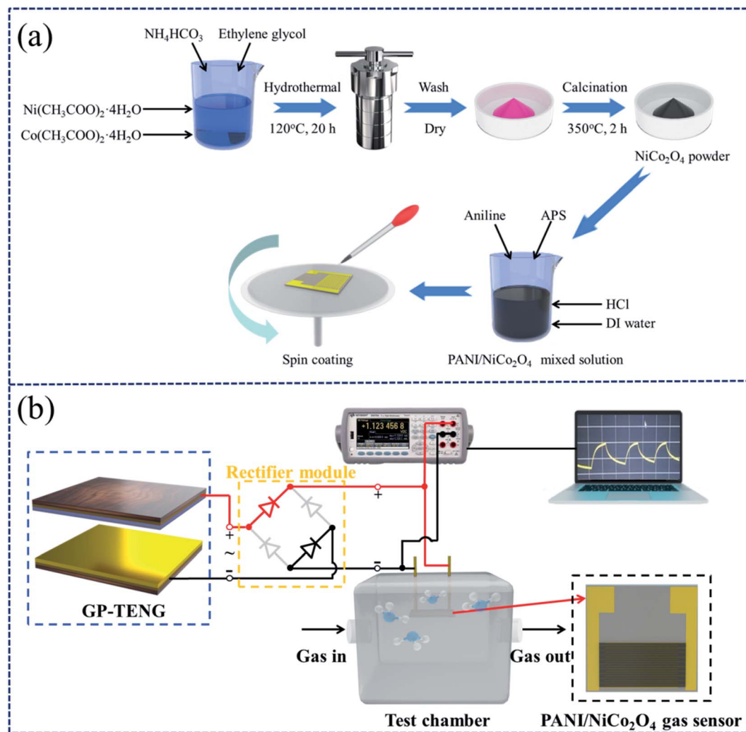
Fig. 2 (a) The diagram of preparation process of the \text{NH}_3 gas sensor based on the PANI/ \text{NiCo}_2\text{O}_4 composite. (b) The experimental test platform of the self-powered GPAS based on the PANI/ \text{NiCo}_2\text{O}_4 composite.
