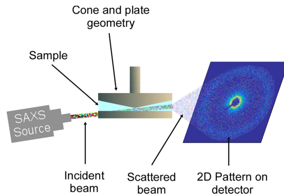
Fig. 1 Schematic of the RheoSAXS setup where X-ray the beam passed through a hole at the bottom plate at a 5^\circ angle and then through the sample capturing the scattering data in the 1\text{--}2 plane.
