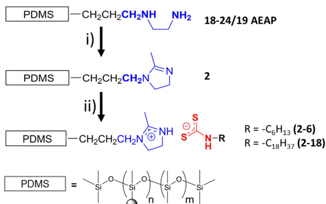
Fig. 2 General pathways for syntheses of PDMS-based ionomers ( R = -C_6H_{13} or -C_{18}H_{37} ) from PDMS-based copolymers with randomly distributed N -propylethylenediamine groups (AEAP): (i) 2.0 M dimethylamine and N,N -dimethylacetamide dimethyl acetal (DMADA) in THF under N_2 at room temperature; (ii) hexylamine or octadecylamine and CS_2 in CHCl_3 at 0 °C. The filled black sphere represents an imidazolium group on a PDMS backbone; n = 18 –24% of the monomer units within a chain.
