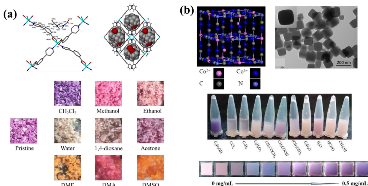
Fig. 3 (a) Coordination environment of Co(II), packing of [\text{Co}(\text{3,4pba})_2] \cdot (\text{H}_2\text{O})_n \cdot 1/2\text{DMF} \cdot \text{H}_2\text{O} ; and pictures of powdered samples after exposure to different solvents. Figures adapted from ref. 126. (b) Structure of \text{Co}_3[\text{Co}(\text{CN})_6]_2 and TEM image of the nanoparticles; the colour of \text{Co}_3[\text{Co}(\text{CN})_6]_2 films changes from pink to purple gradually with an increasing ethanol concentration gradient. Adapted with permission from ref. 96.
