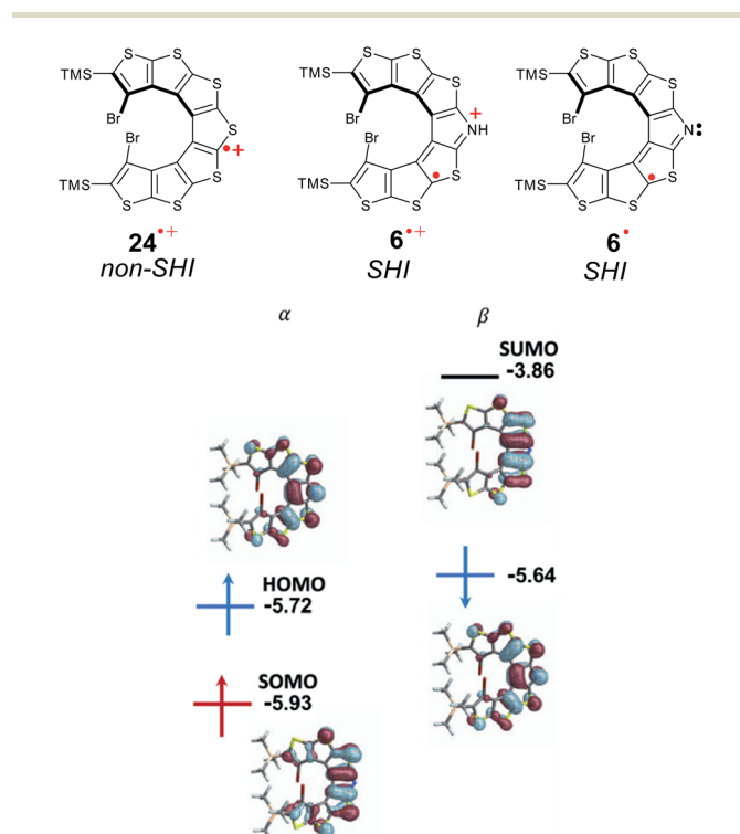
Fig. 16 Chemical structures of cationic radicals thia[7]helicene 24^{+\cdot}[\text{PF}_6]^- and aza-thia[7]helicene 6^{+\cdot}[\text{PF}_6]^- , and neutral aza-thia[7]helicene 6^{\cdot} . Orbital energies (in eV) and isosurfaces ( \pm 0.030 a.u.) of selected MOs of 7 . Figures adapted with permission from ref. 53. Copyright 2021 American Chemical Society.
