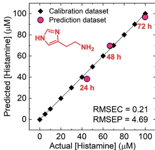
Fig. 6 Real sample analysis using SVM for freshness monitoring of the raw fish [S1–S3] = 1.2 \times 10^{-4} g mL ^{-1} . The target histamine was extracted from the raw fish (tuna) stored for 24 h, 48 h, and 72 h at 25 °C. The values of the root-mean-square of calibration (RMSEC) and prediction (RMSEP) prove the high accuracy of the model and its predictive capacity. The actual concentrations of histamine in the fish sample were determined by HPLC.
