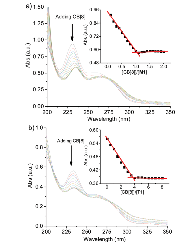
Fig. 2 UV-vis absorption spectra of (a) M1 (20 \mu\text{M} ) and (b) T1 (2.5 \mu\text{M} ) in water in the presence of an incremental amount of CB[8] at 25 °C. Inset: the absorbance at 233 nm vs. [\text{CB}[8]]/[\text{M1}] or [\text{T1}] .
