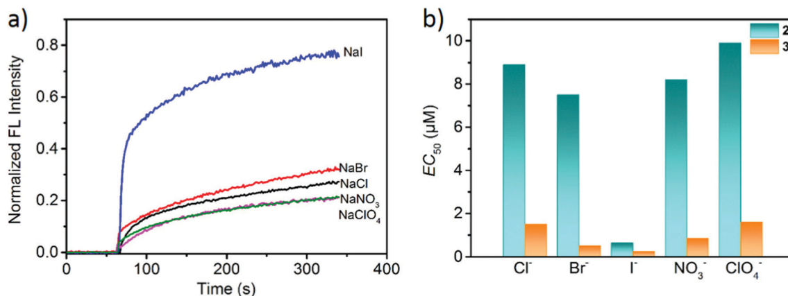
Fig. 8 (a) Transport activities toward \text{Cl}^- , \text{Br}^- , \text{I}^- , \text{NO}_3^- and \text{ClO}_4^- at a final concentration of 1 \mu\text{M} for 2 (2:lipid = 1:375). The background rates of \text{I}^- and \text{ClO}_4^- were subtracted. (b) The \text{EC}_{50} values for 2 and 3 mediated transport of \text{Cl}^- , \text{Br}^- , \text{I}^- , \text{NO}_3^- and \text{ClO}_4^- determined using the HPTS assay.
