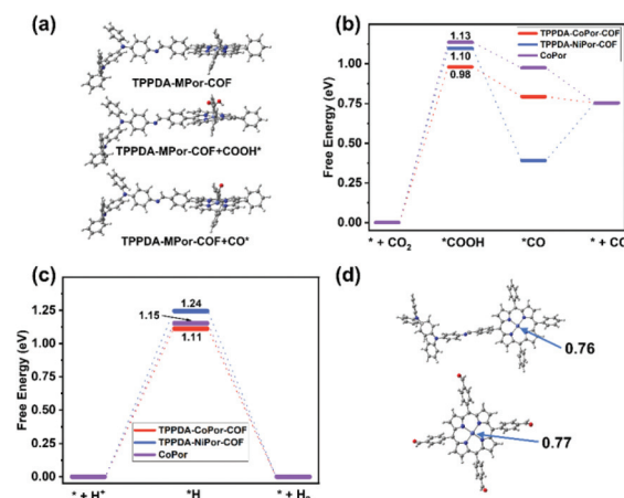
Fig. 7 (a) The proposed mechanism of the electrocatalytic CO 2 RR for TPPDA-MPor-COFs. (b) The calculated energy diagrams of CO 2 reduction to CO and (c) the calculated energy diagrams of the HER for TPPDA-MPor-COFs and CoPor. (d) The Mulliken charge of the Co site in TPPDA-MPor-COF and CoPor.
