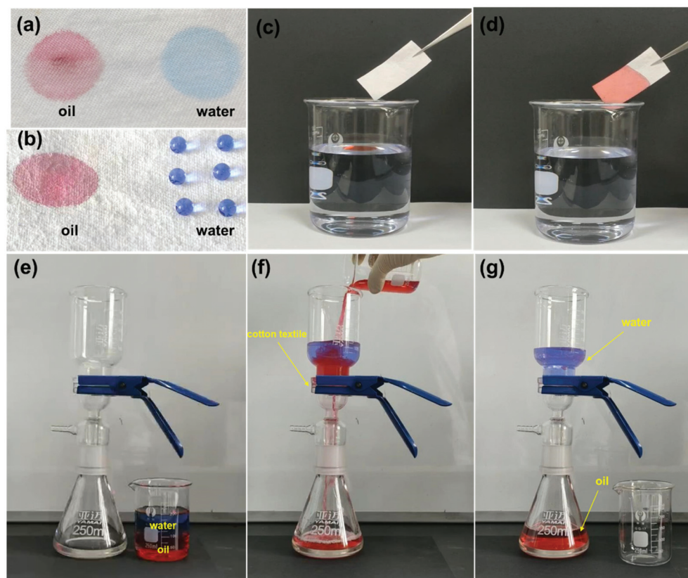
Fig. 8 Pictures of oil and water droplets on (a) the pure cotton fabric and (b) the SiO 2 -TiO 2 /PDMS-coated superhydrophobic cotton fabric. (c and d) Pictures of the absorbing process of n -hexane (dyed with Sudan IV) from water. (e–g) The dichloromethane–water mixture separation test of SiO 2 -TiO 2 /PDMS-coated superhydrophobic cotton fabric.
