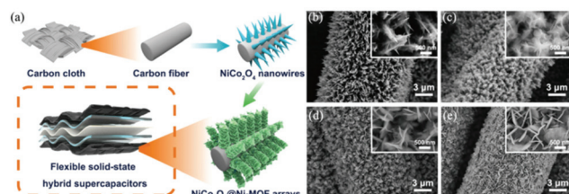
Fig. 4 (a) Schematic illustration of the synthesis of \text{NiCo}_2\text{O}_4@\text{Ni-MOF} on CF. (b–e) SEM images of \text{NiCo}_2\text{O}_4@\text{Ni-MOF} synthesized at 3, 6, 12, and 24 h for MOF growth, respectively. Reprinted with permission from ref. 58, Copyright 2019, American Chemical Society.
